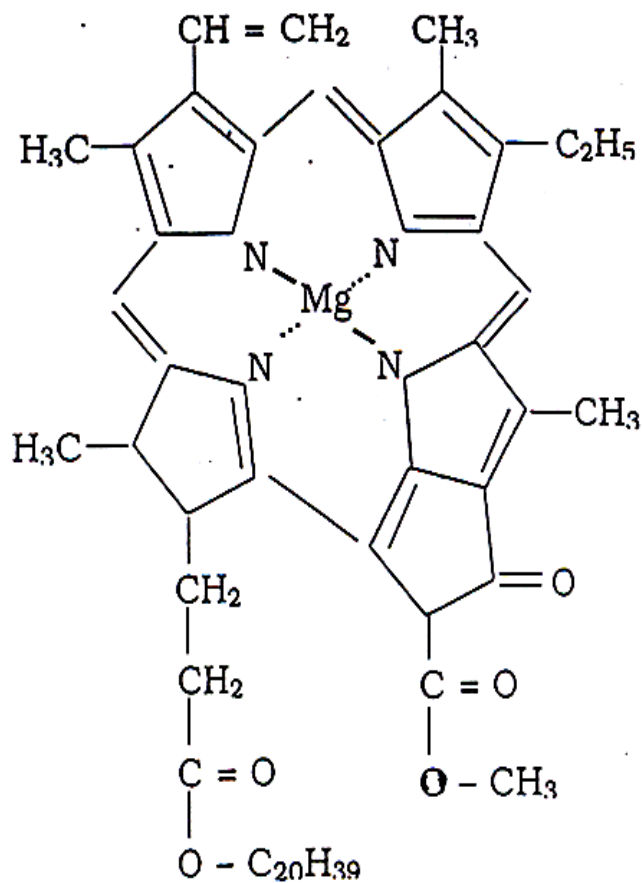
C_{55}H_{72}O_5N_4Mg (a)
