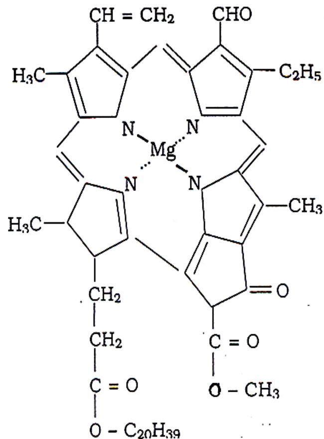
C_{55}H_{70}O_6N_4Mg (b)
