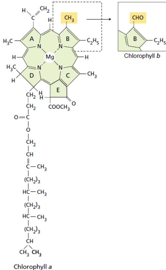
(A) Chlorophylls
